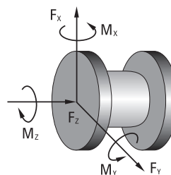
Figure 53. Right-handed Orthogonal Coordinate System
