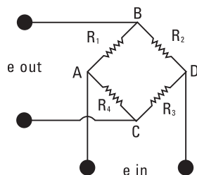
Figure 50. Wheatstone Bridge
