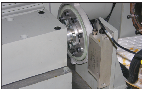
TORKDISC® Rotary Torque Sensor System
