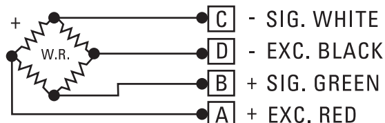
Figure 48. Load Cell Wiring Code
