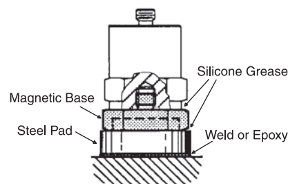
Figure 24. Magnet Mounted to Steel Pad
