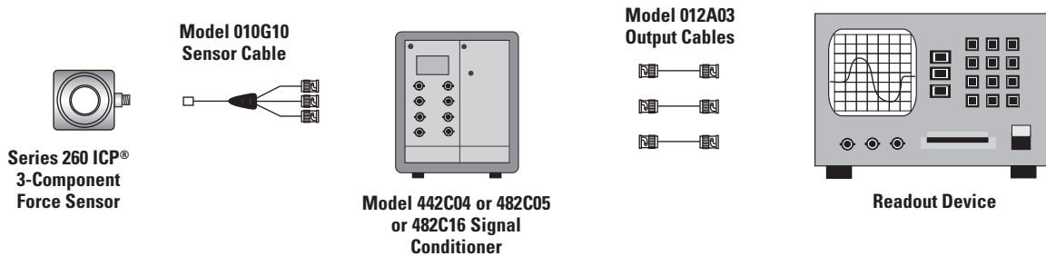
Figure 42. System Utilizing a ICP® Sensor Signal Conditioner
