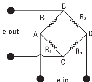
Figure 47. Wheatstone Bridge
