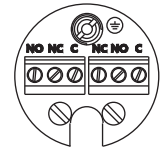
TERMINAL CONNECTIONS DPDT
