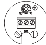
TERMINAL CONNECTIONS SPDT
