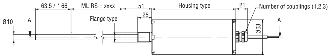
Type 1 Cable outlet Housing type 1 = 150
