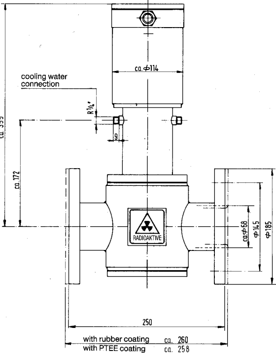
Flanged density measuring system
